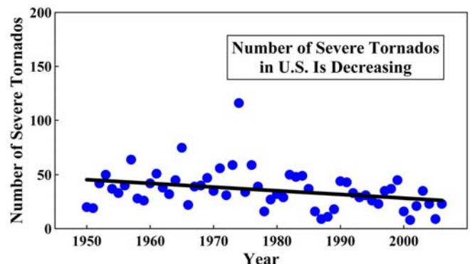
Figure 8: Annual number of strong-to-violent category F3 to F5 tornadoes during the March-to-August tornado season in the U.S. between 1950 and 2006. U.S. National Climatic Data Center, U.S. Department of Commerce 2006 Climate Review (20). During this period, world hydrocarbon use increased 6-fold, while violent tornado frequency decreased by 43%.
